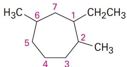
1-Ethyl-2,6-dimethylcycloheptane
