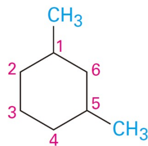
1,5-Dimethylcyclohexane
