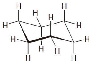
Cyclohexane (chair conformation)
