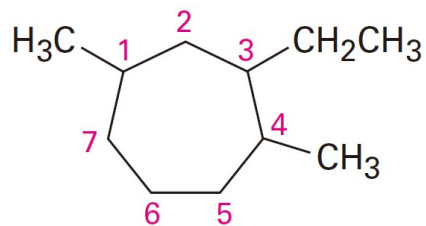
3-Ethyl-1,4-dimethylcycloheptane
