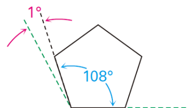
Cyclopentane
