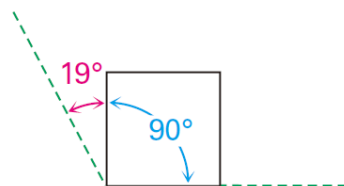
Cyclobutane
