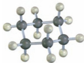
Cyclohexane (chair conformation)
