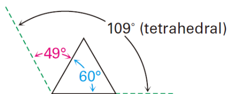
Cyclopropane
