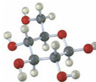
Glucose (chair conformation)
