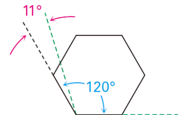
Cyclohexane
